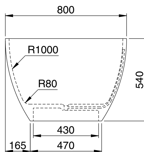
Side View - Section View
