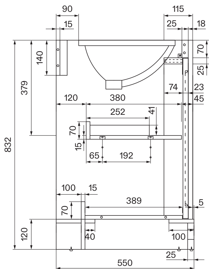
Side View - Section View
