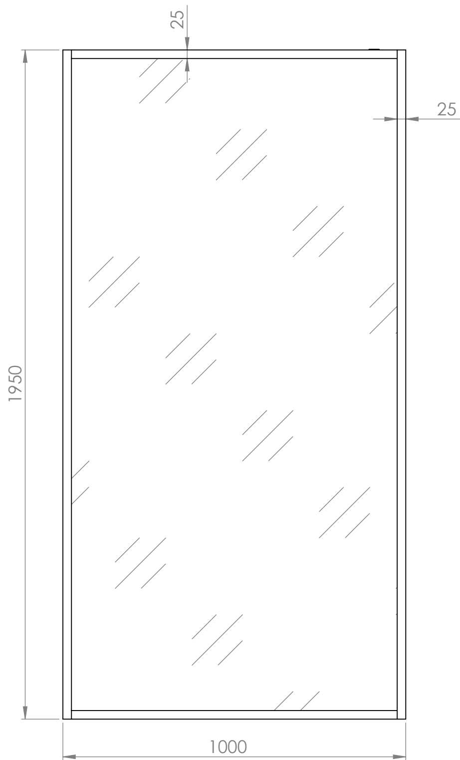
Front View
