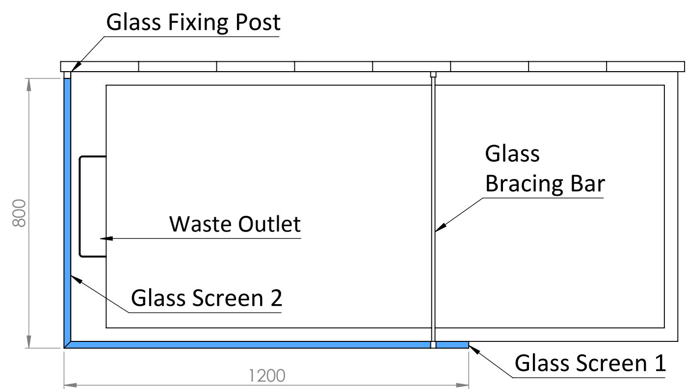
Shower Tray with Enclosure Kit - A
