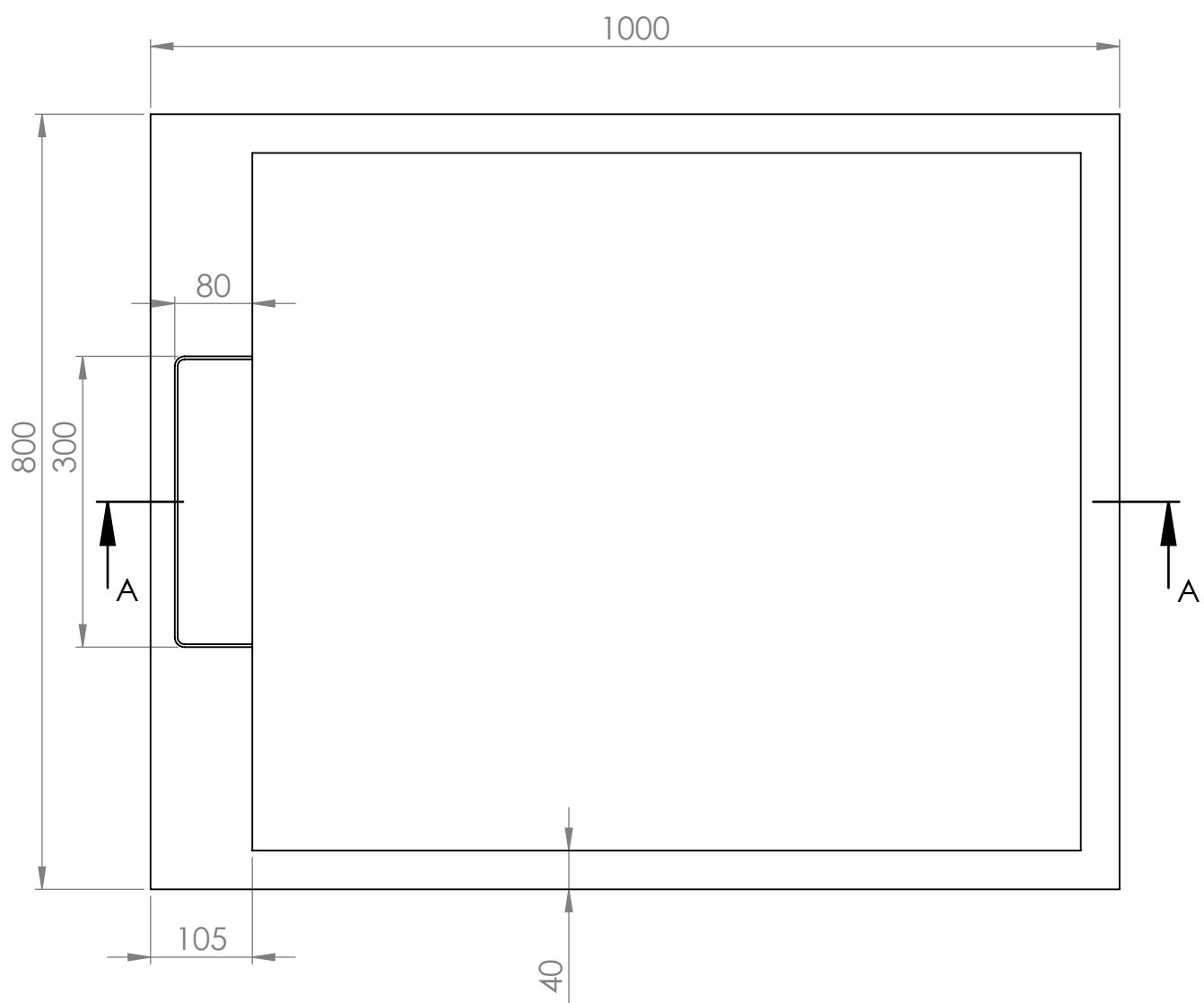
Shower Tray - Top View
