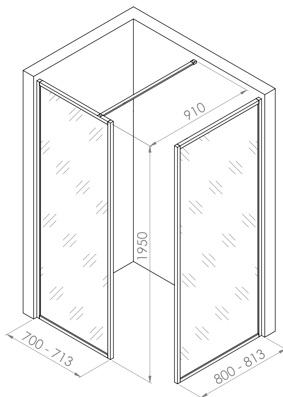
Full Enclosure View
