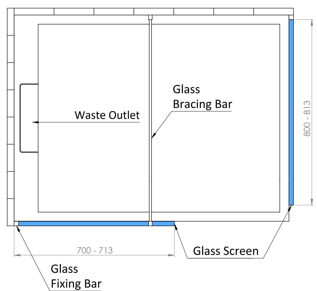
Shower Tray with Enclosure Kit - B
