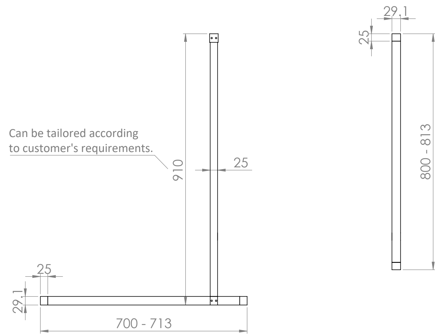
Shower Tray with Enclosure Kit - B
