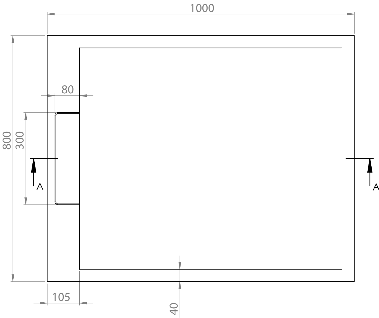
Shower Tray - Top View
