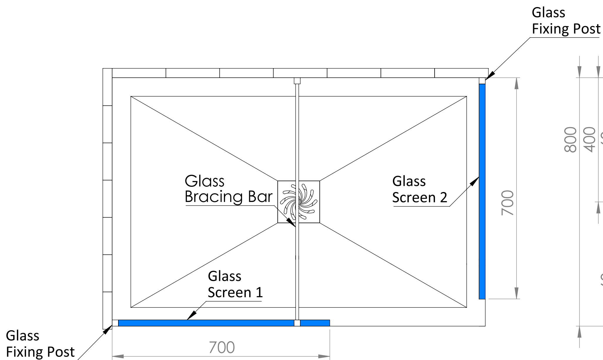
Shower Tray with Enclosure Kit - A
