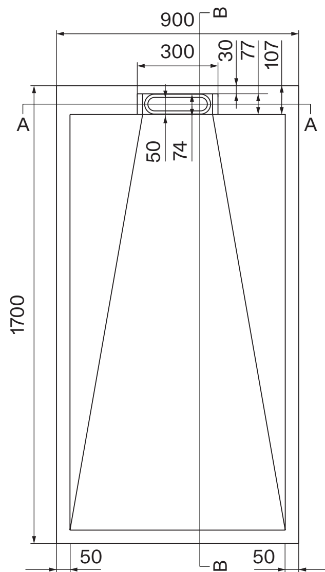
Top View
