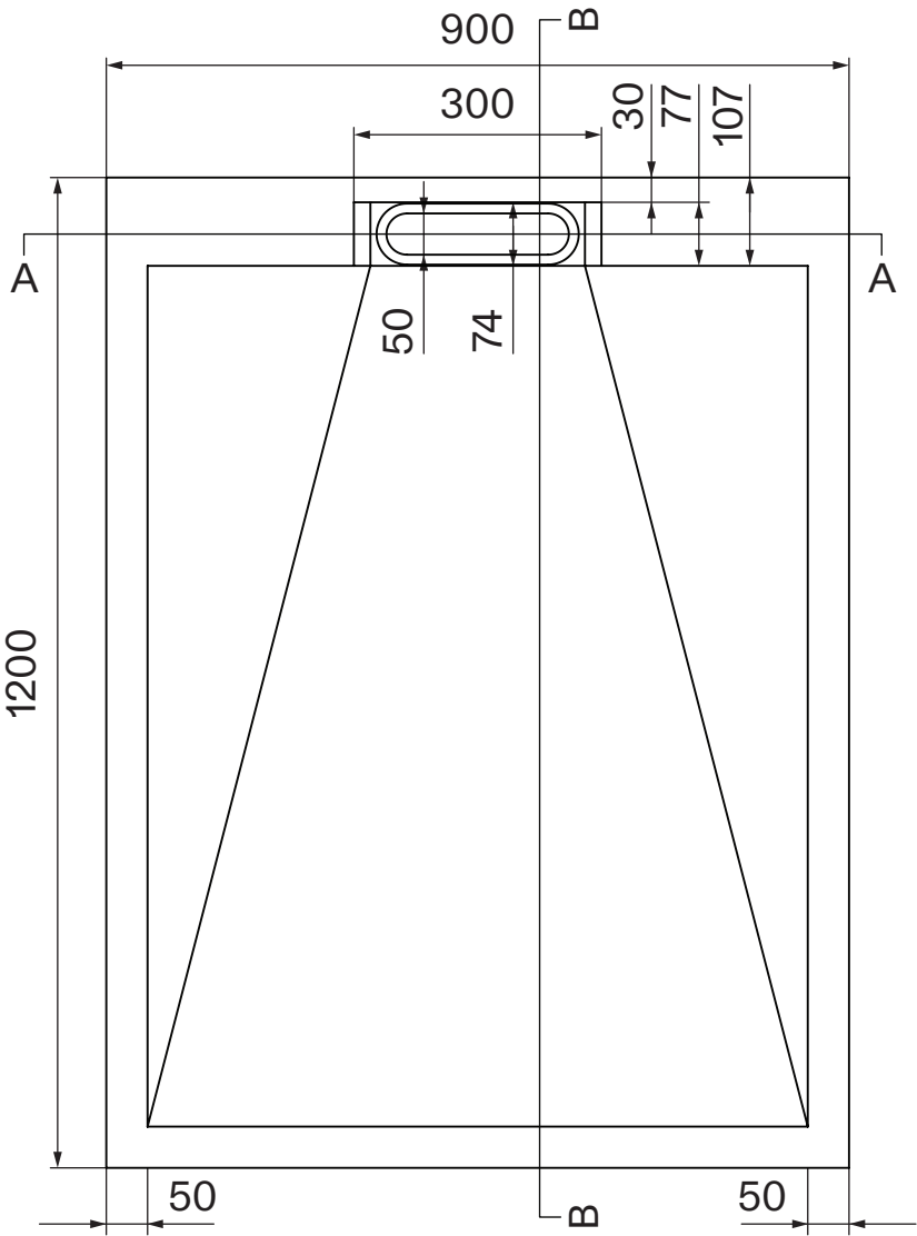
Top View
