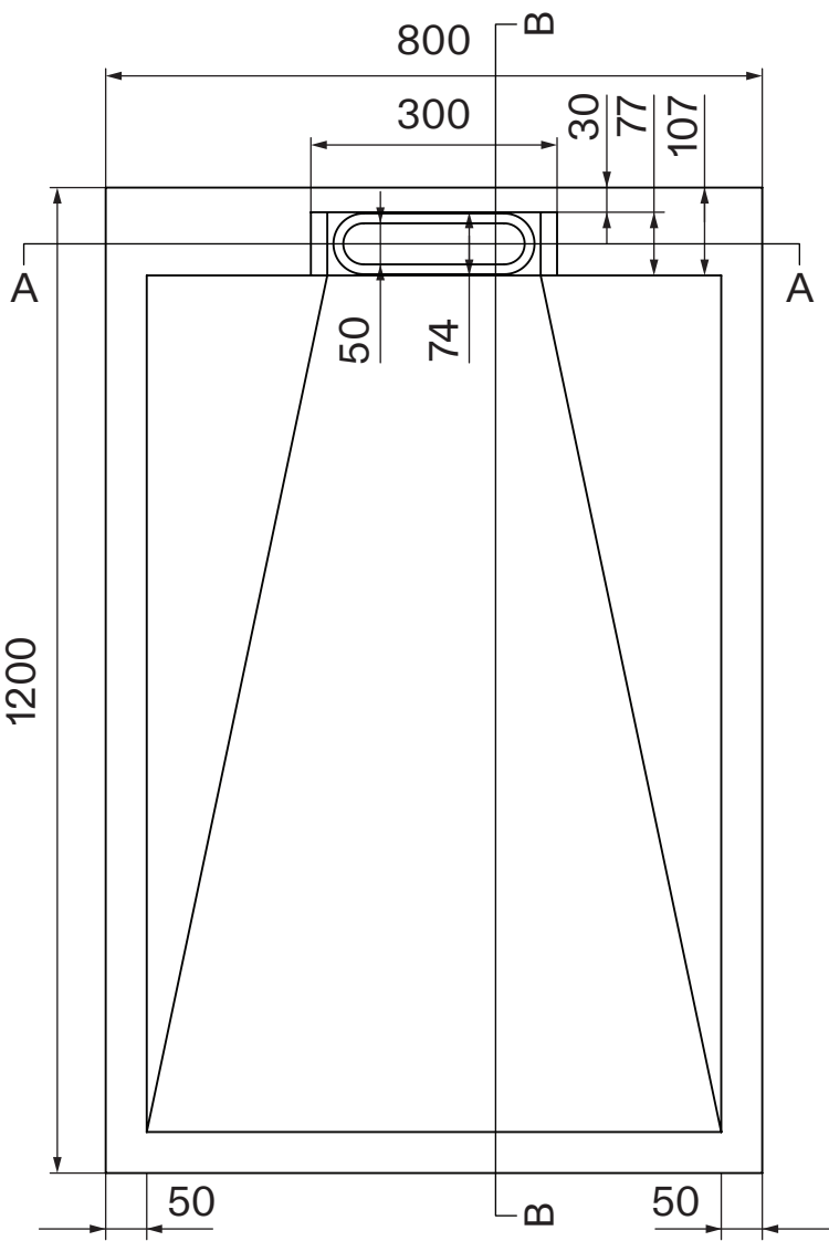
Top View
