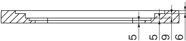
Section C
