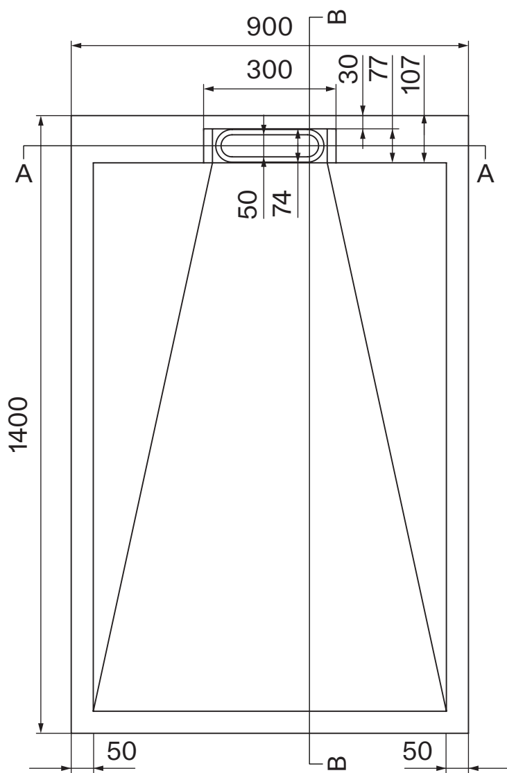
Top View
