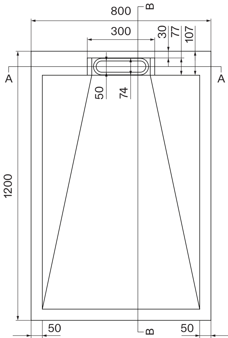
Top View
