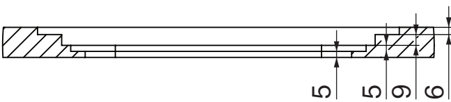
Section C
