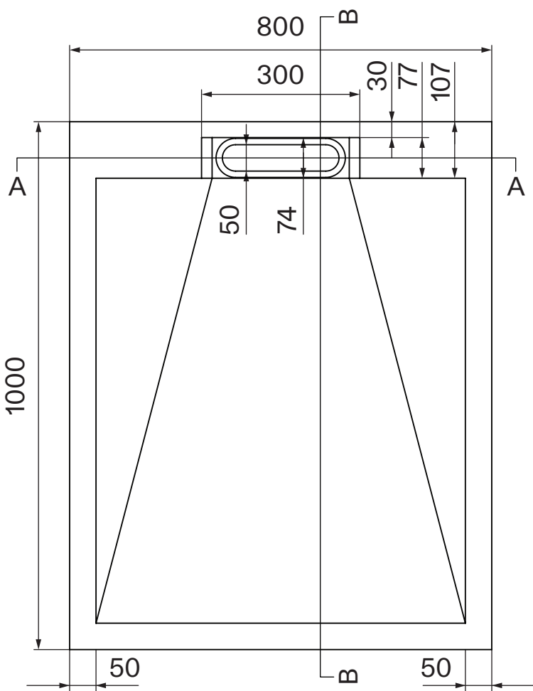
Top View
