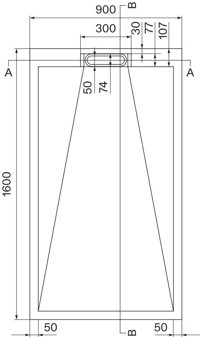
Top View
