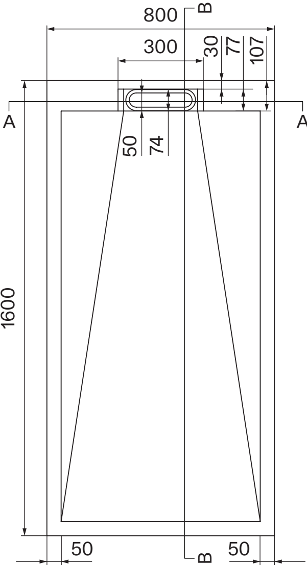
Top View
