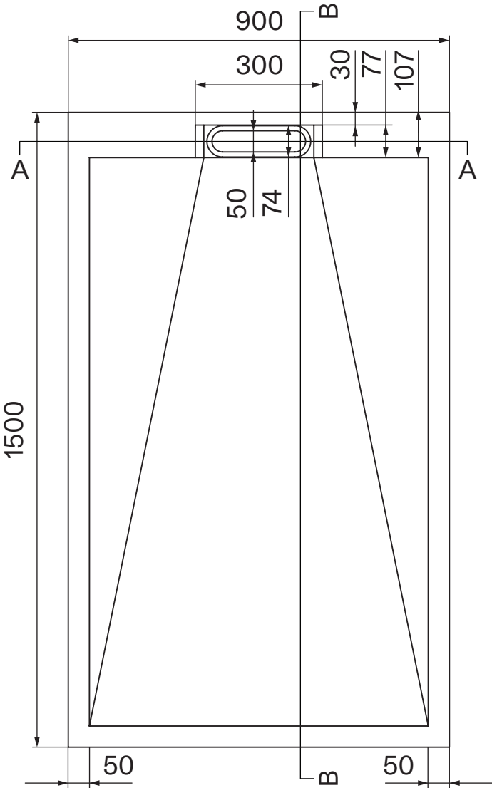
Top View
