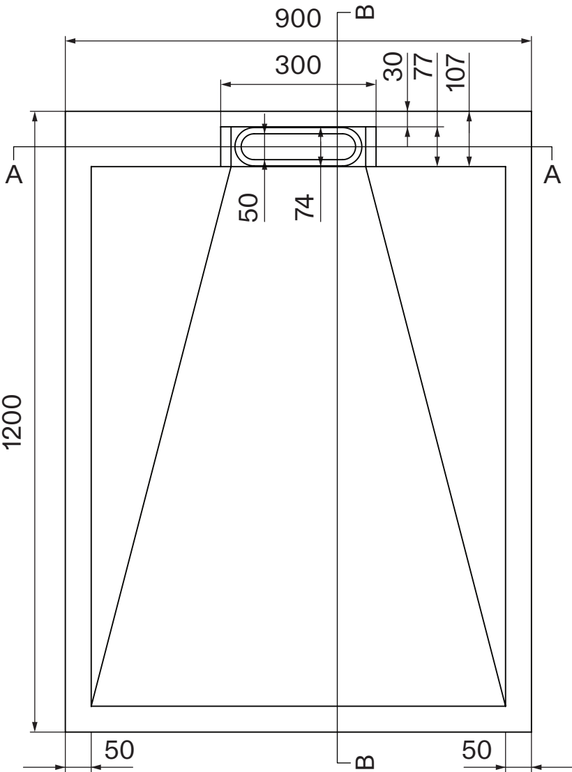
Top View
