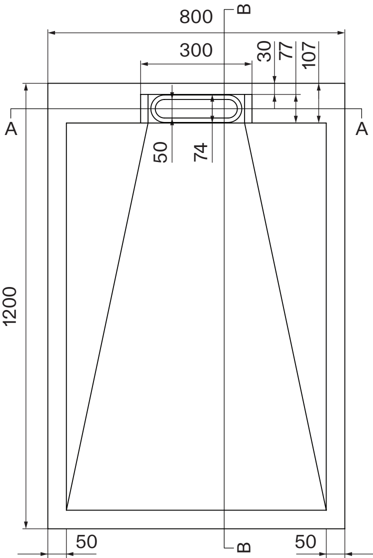
Top View
