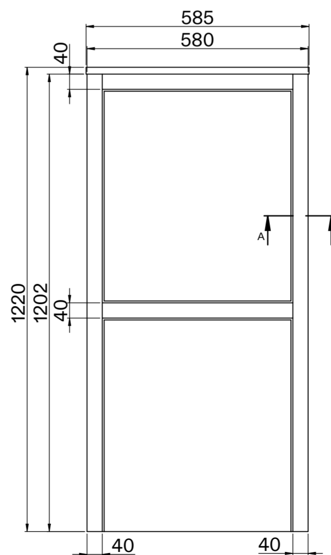
Front View
