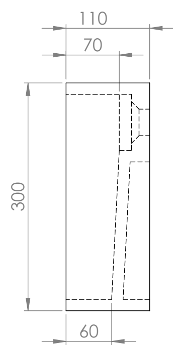
Side View - Section View
