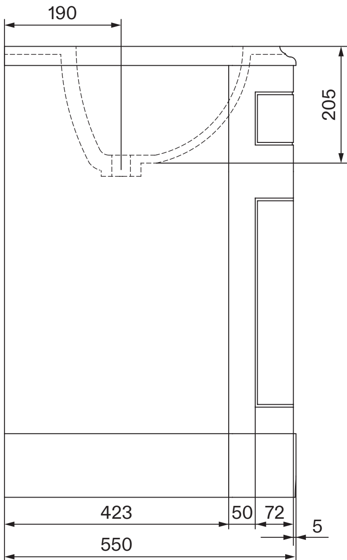
Side View
