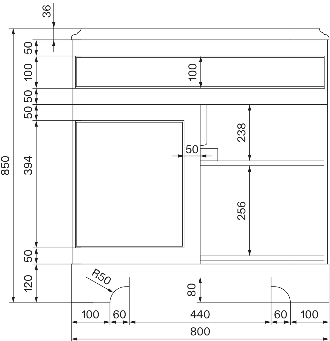
Front View
