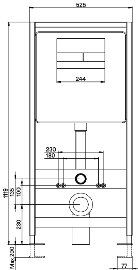
Front View
