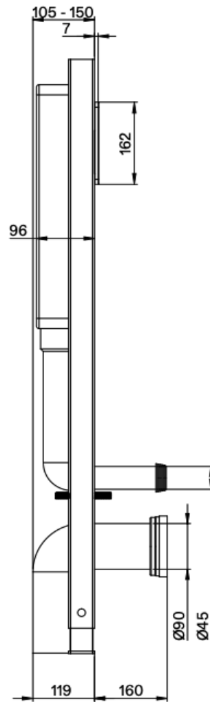
Side View
