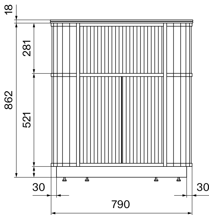
Front View - Vanity Unit
