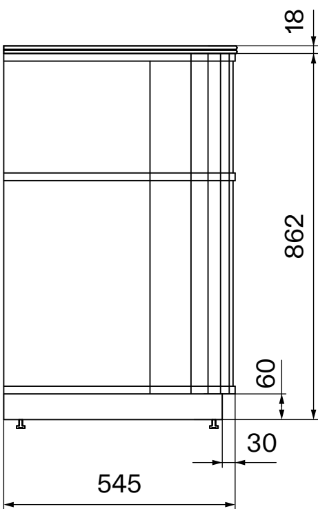
Side View - Vanity Unit
