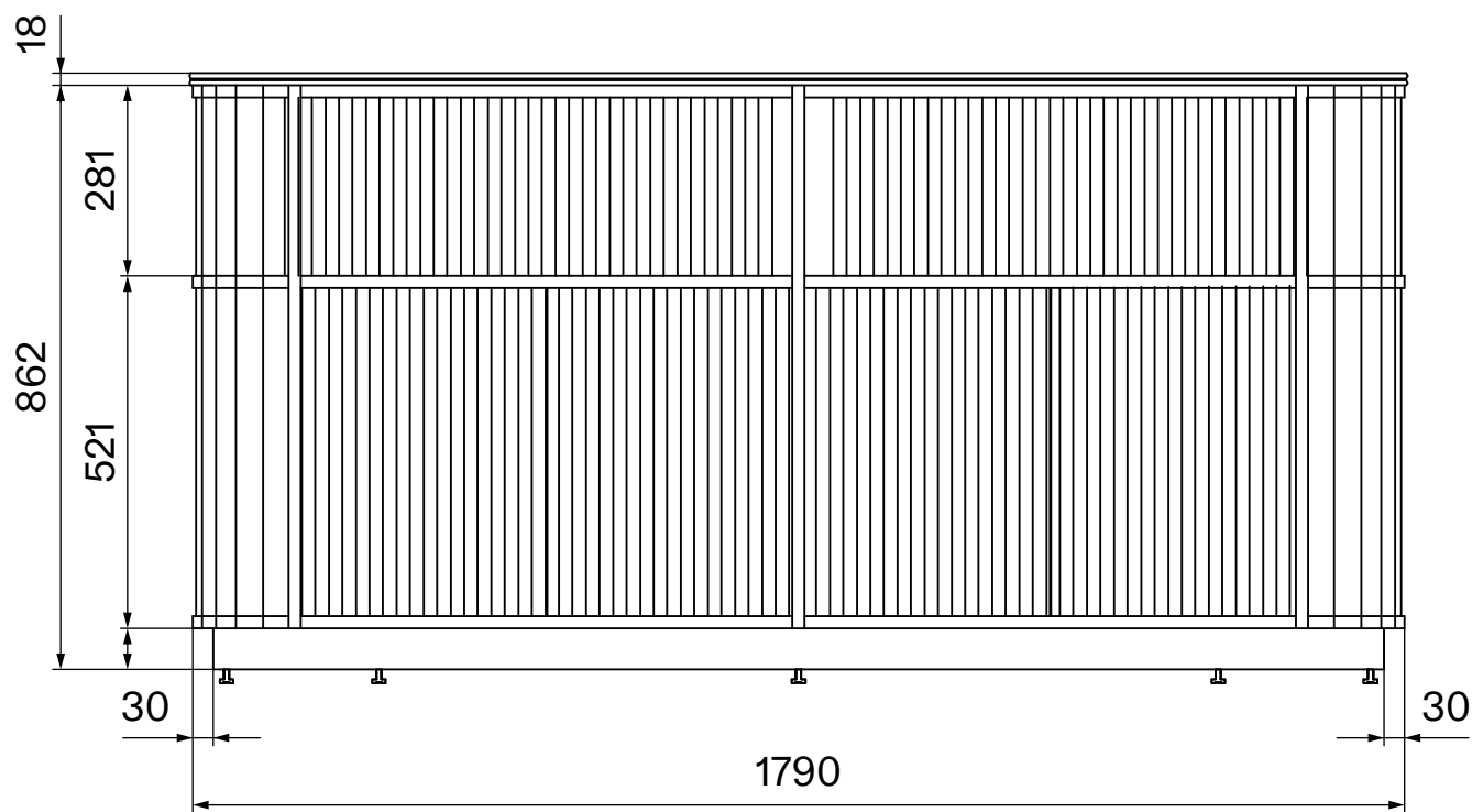
Front View - Vanity Unit
