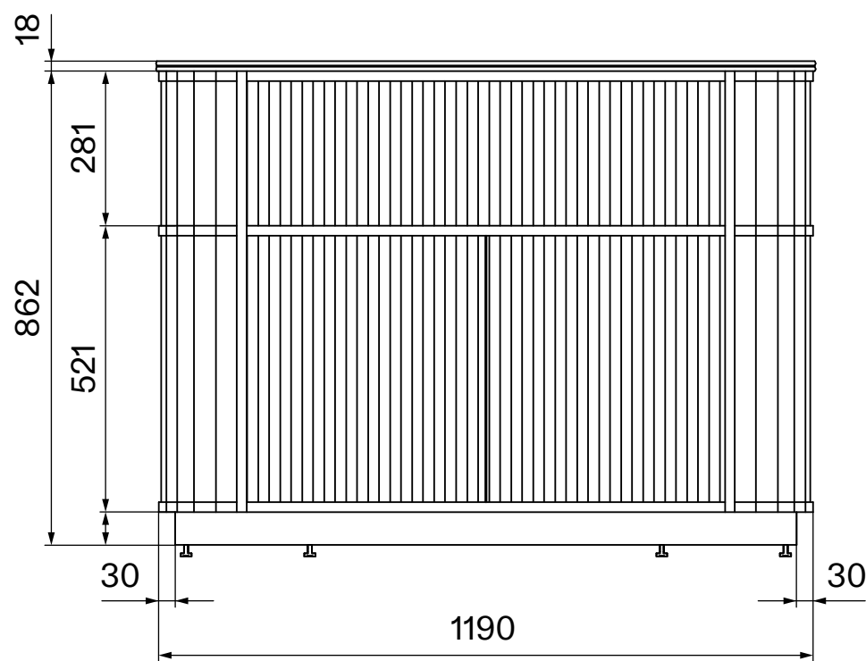
Front View - Vanity Unit
