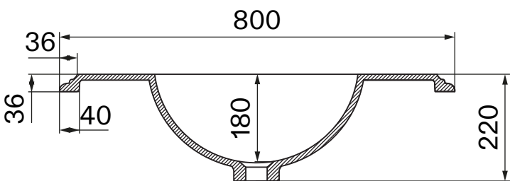
Front View - Section View - Basin
