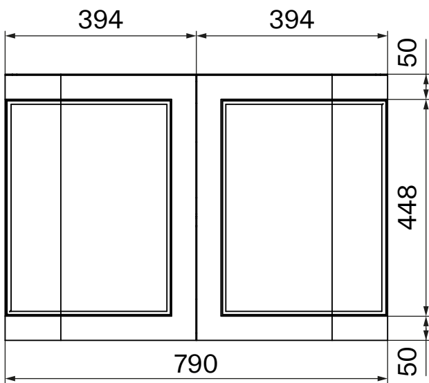
Front View - Vanity
