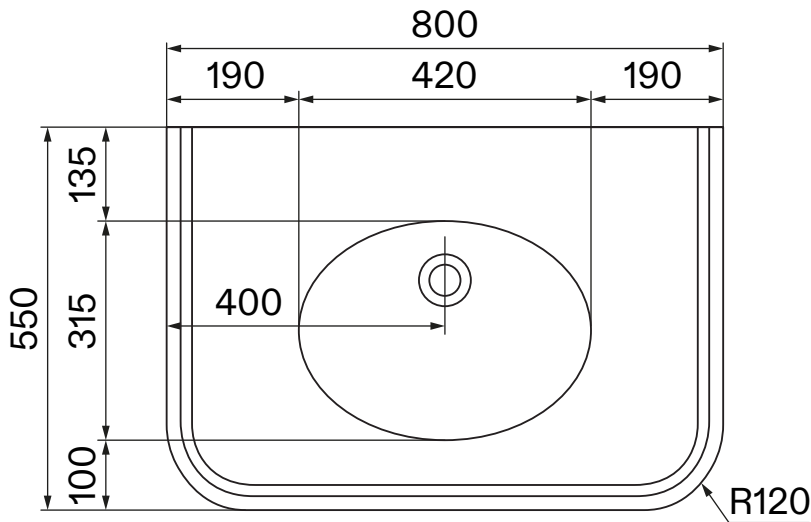
Front View - Section View - Basin
