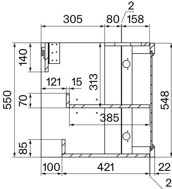
Side View - Section View - Vanity
