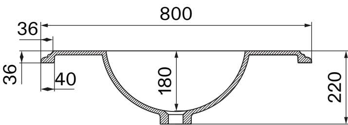
Front View - Section View - Basin
