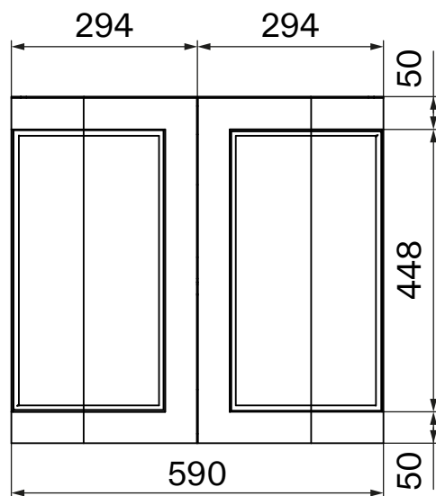
Front View - Vanity
