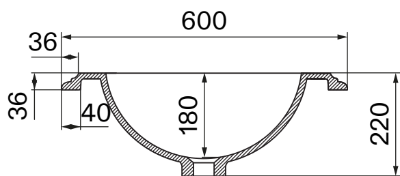
Front View - Section View - Basin
