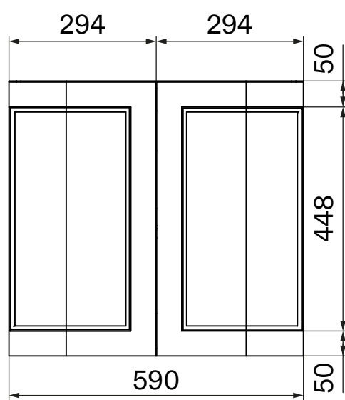
Front View - Vanity
