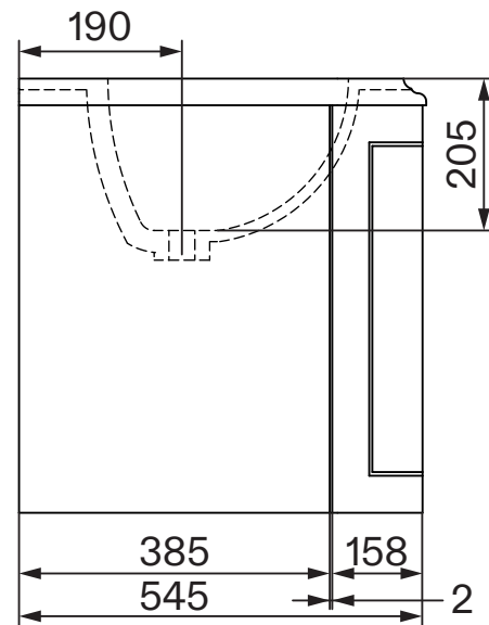
Side View - Basin and Vanity
