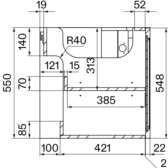
Side View - Section View - Vanity
