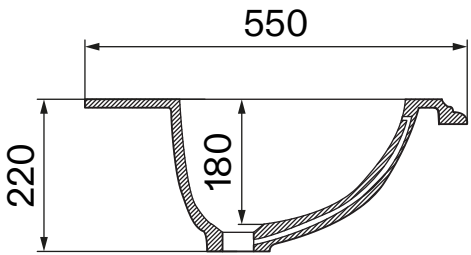
Side View - Section View - Basin
