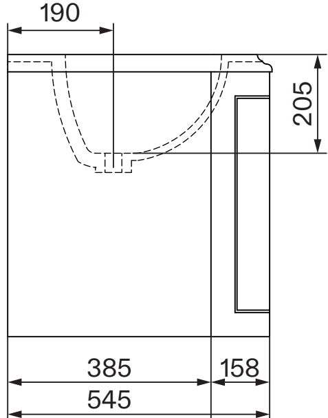
Side View - Basin and Vanity
