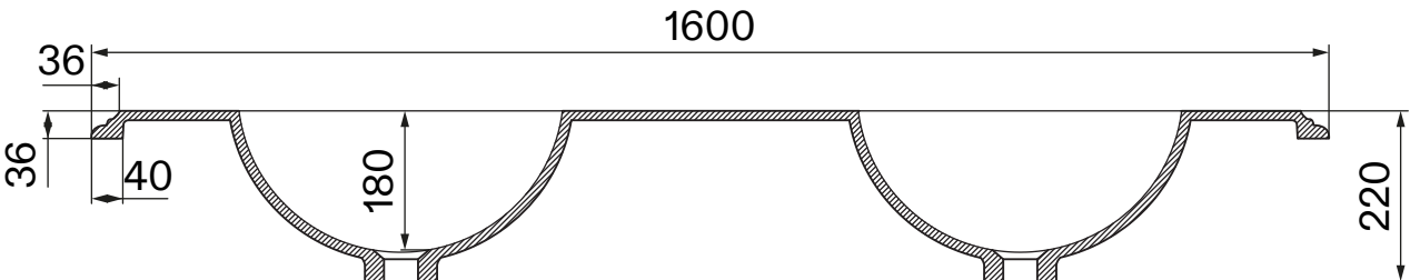
Front View - Section View - Basin
