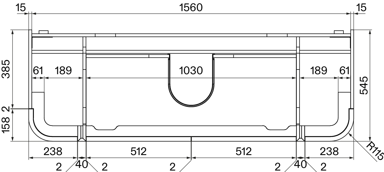
Top View - Section View - Vanity
