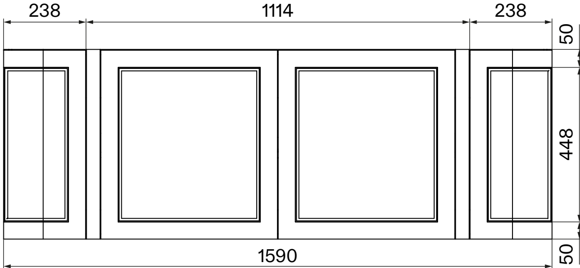
Top View - Section View - Vanity
