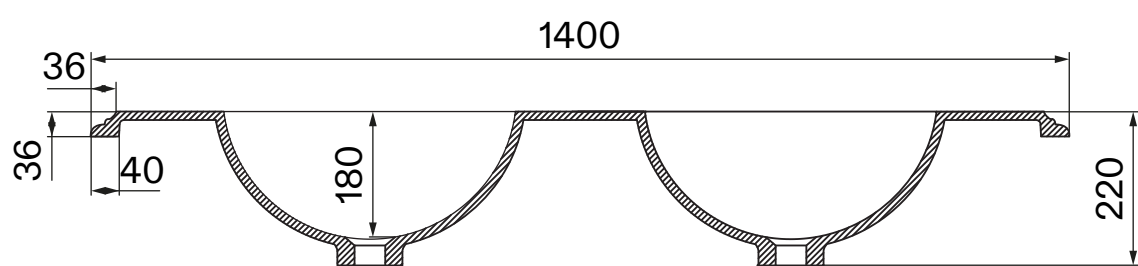
Front View - Section View - Basin
