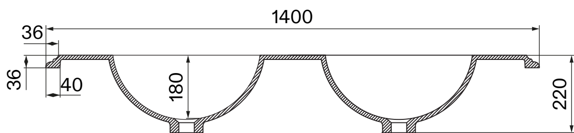
Front View - Section View - Basin
