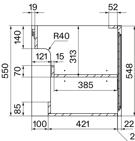
Side View - Section View - Vanity
