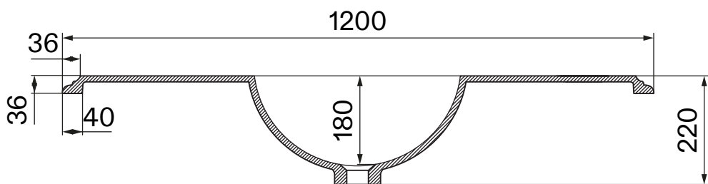
Front View - Section View - Basin
