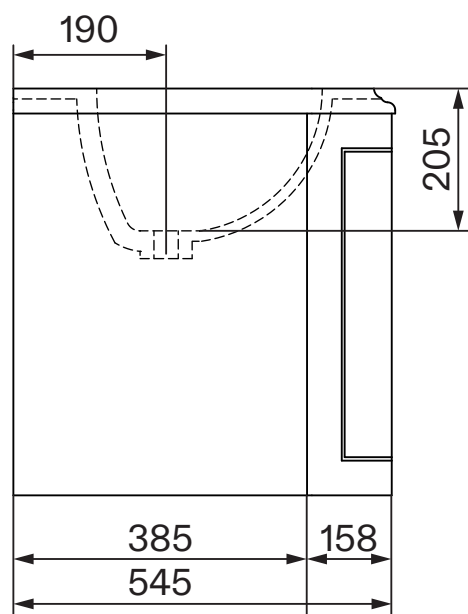
Side View - Basin and Vanity
