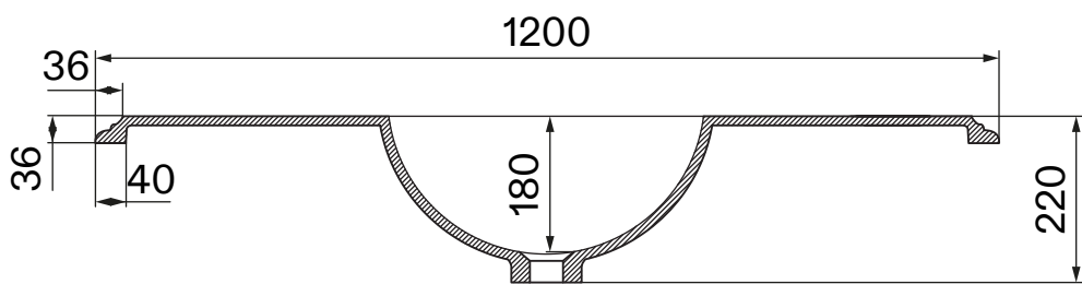
Front View - Section View - Basin
