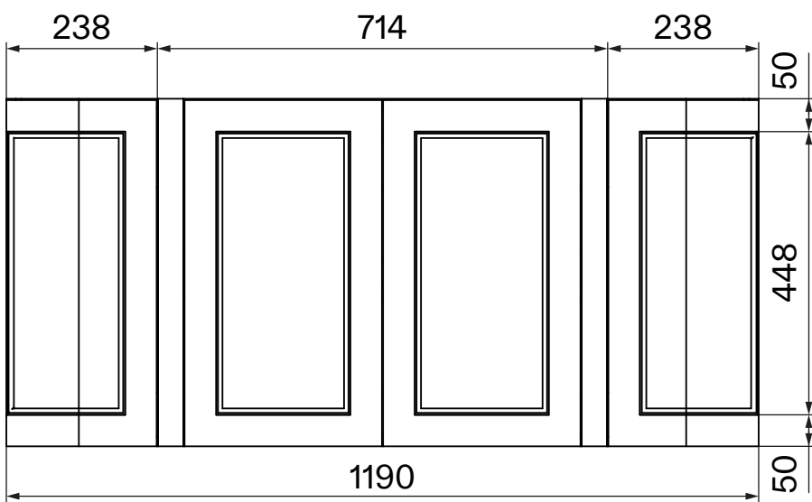
Front View - Vanity
