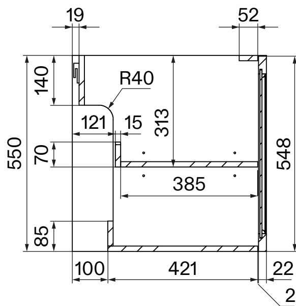
Side View - Section View - Vanity
