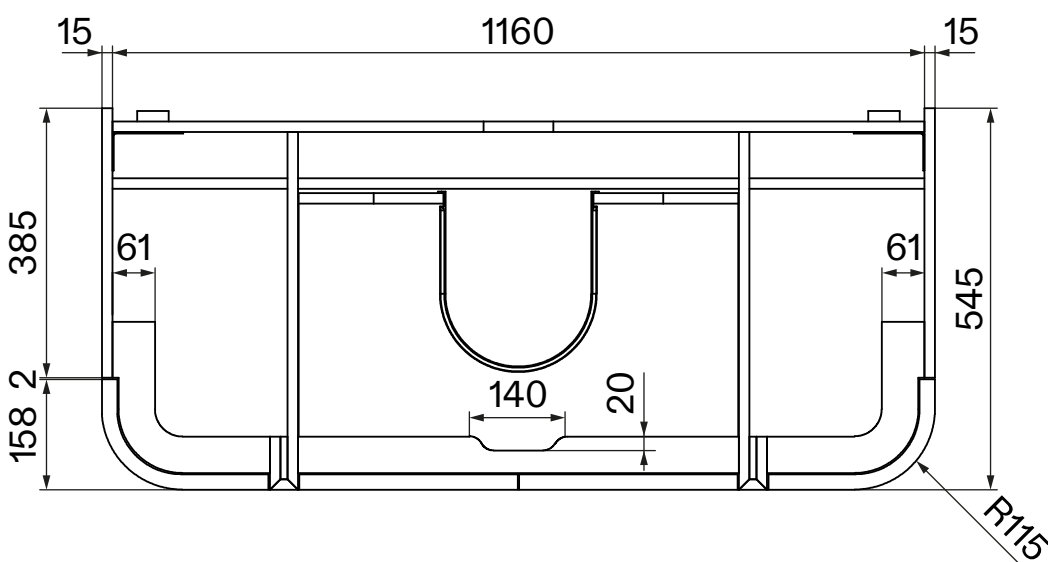
Top View - Section View - Vanity
