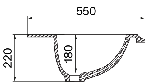
Side View - Section View - Basin
