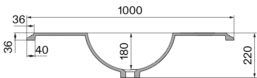
Front View - Section View - Basin
