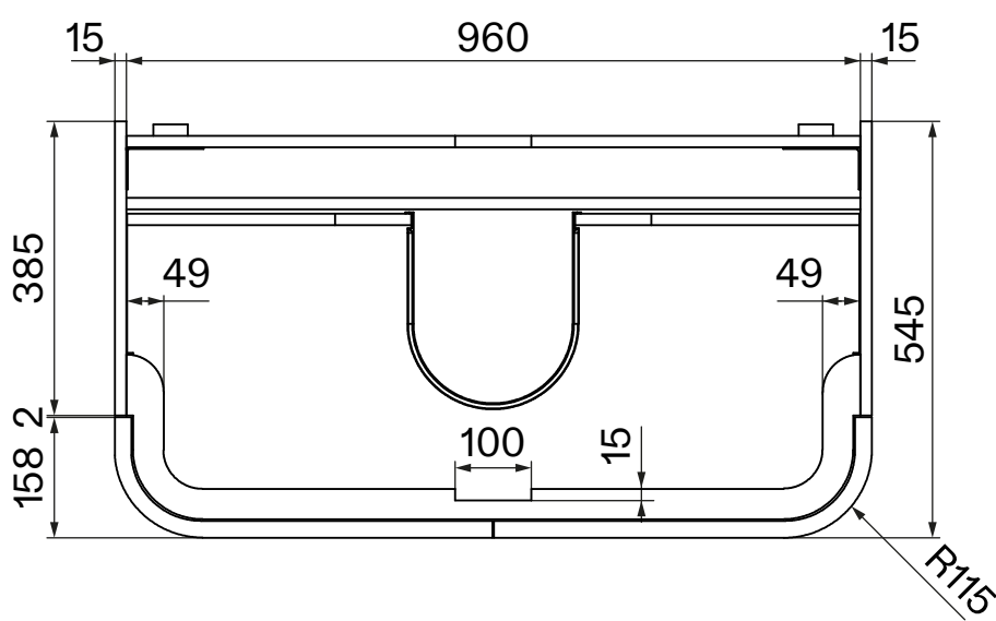
Top View - Section View - Vanity
