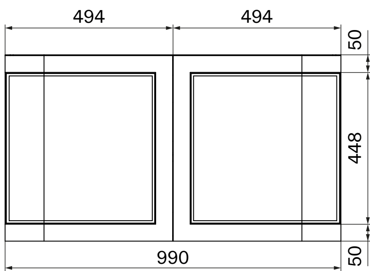
Front View - Vanity
