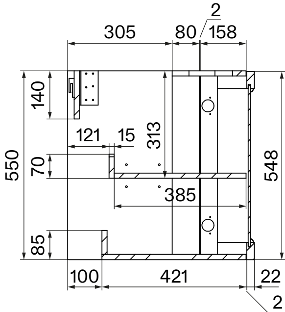
Side View - Section View - Vanity
