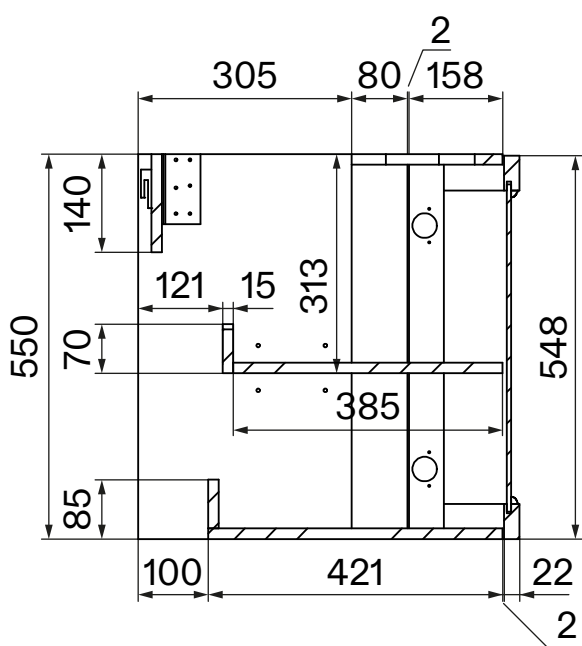
Side View - Section View - Vanity
