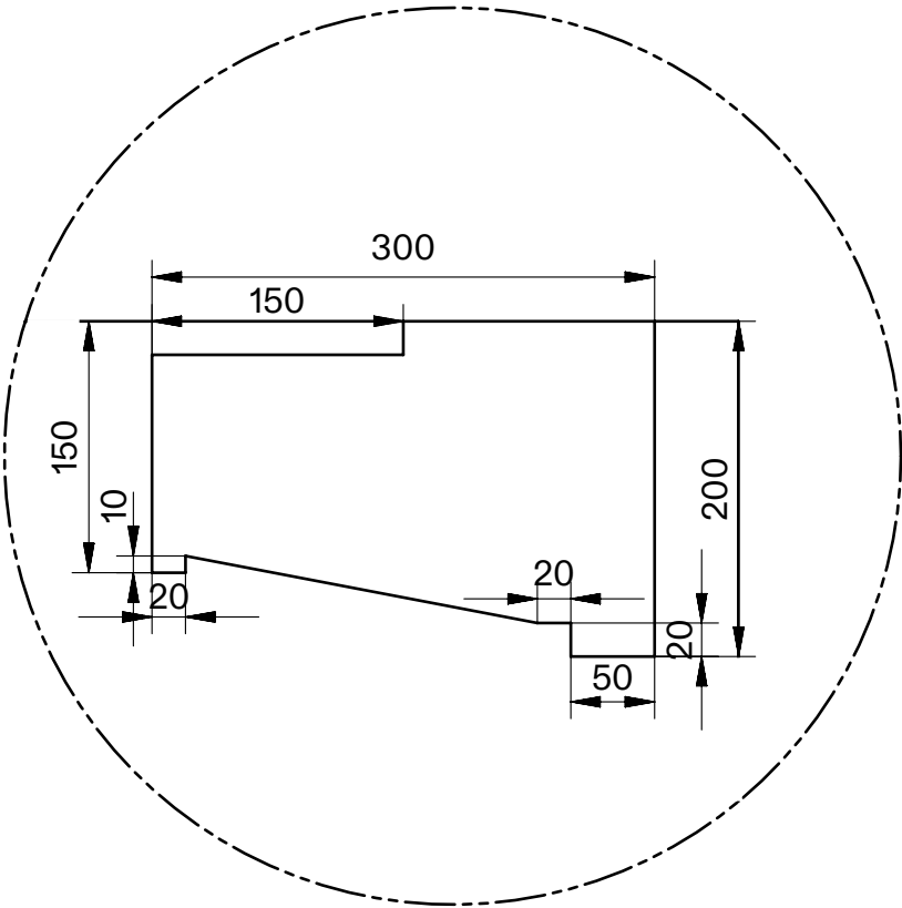
Detail B Scale 1:5
