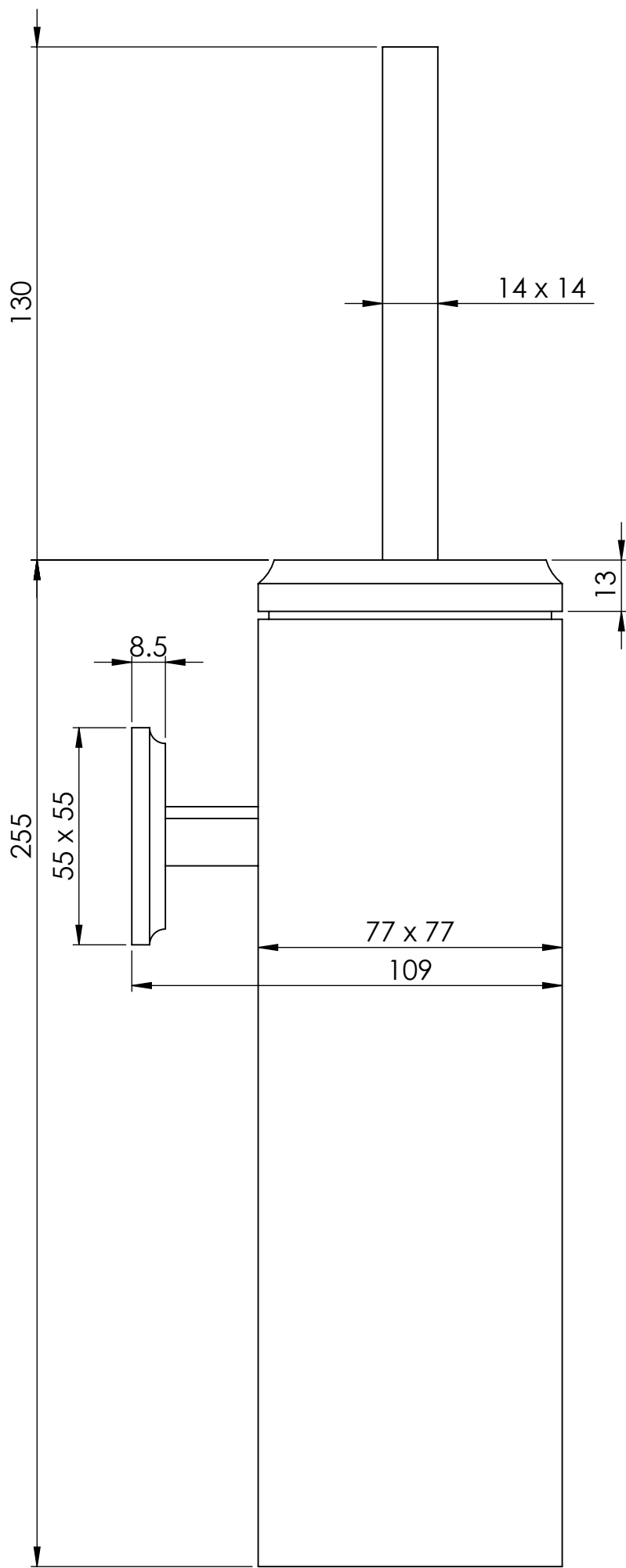
Side View
