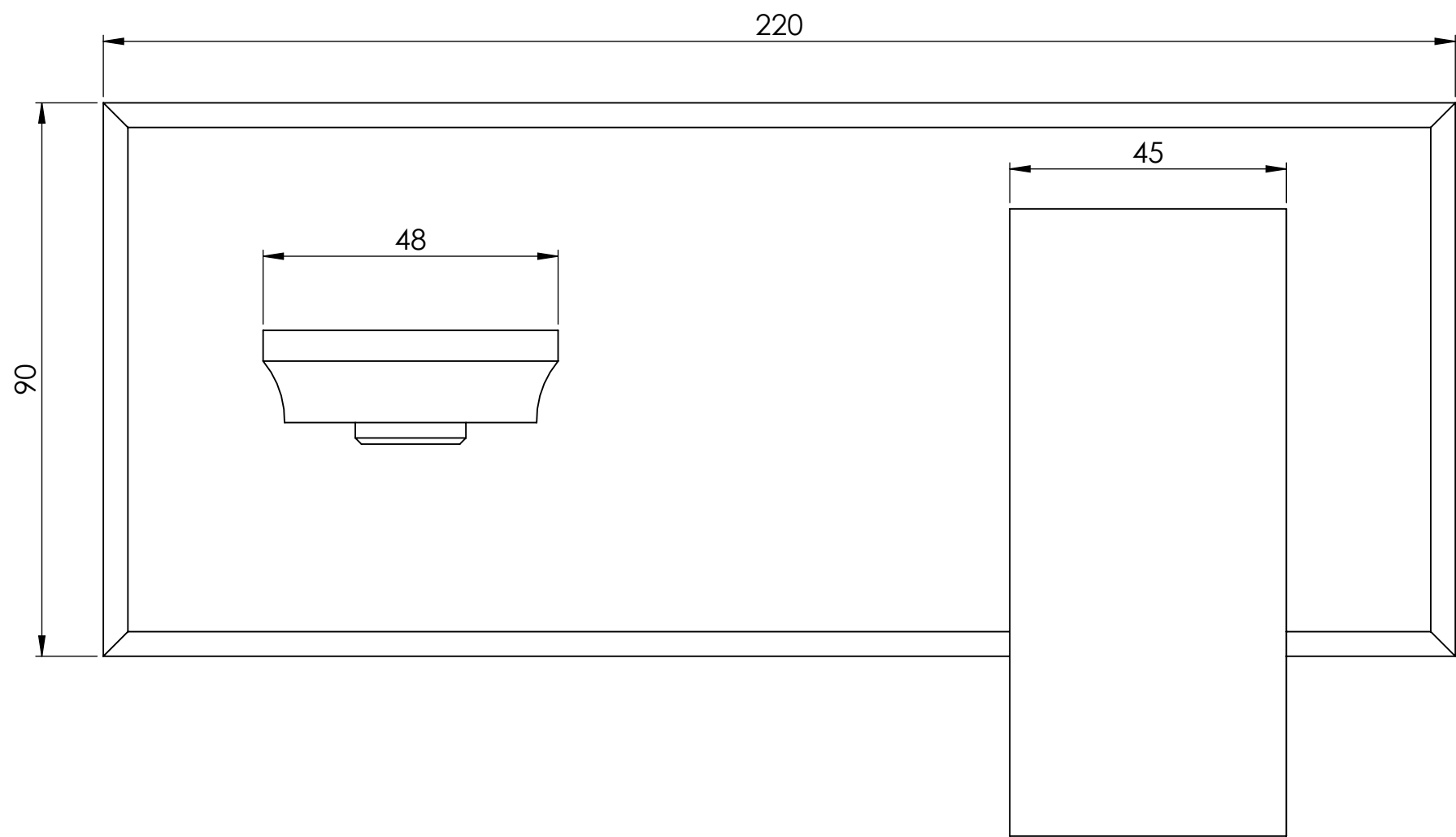
Front View
