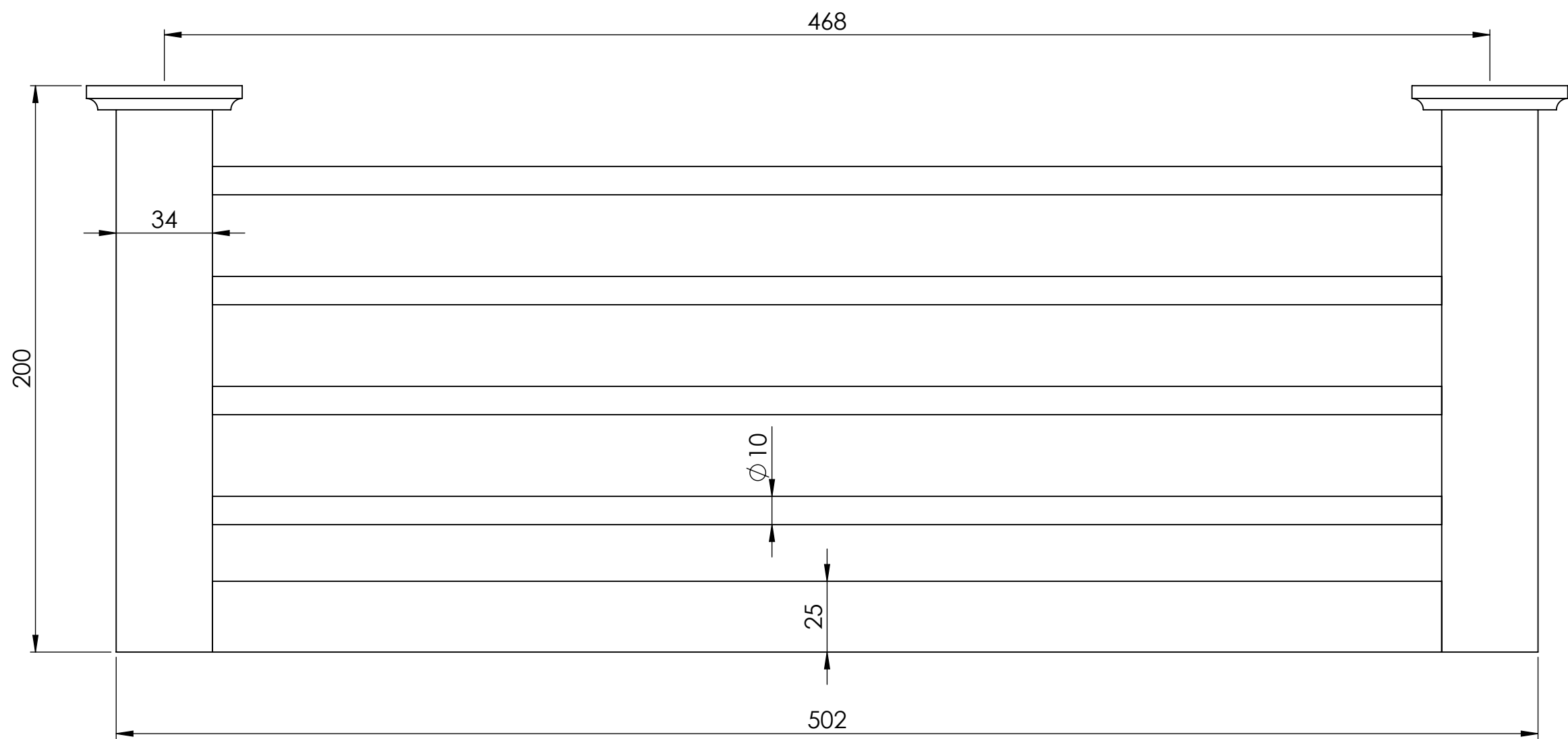
Top View
