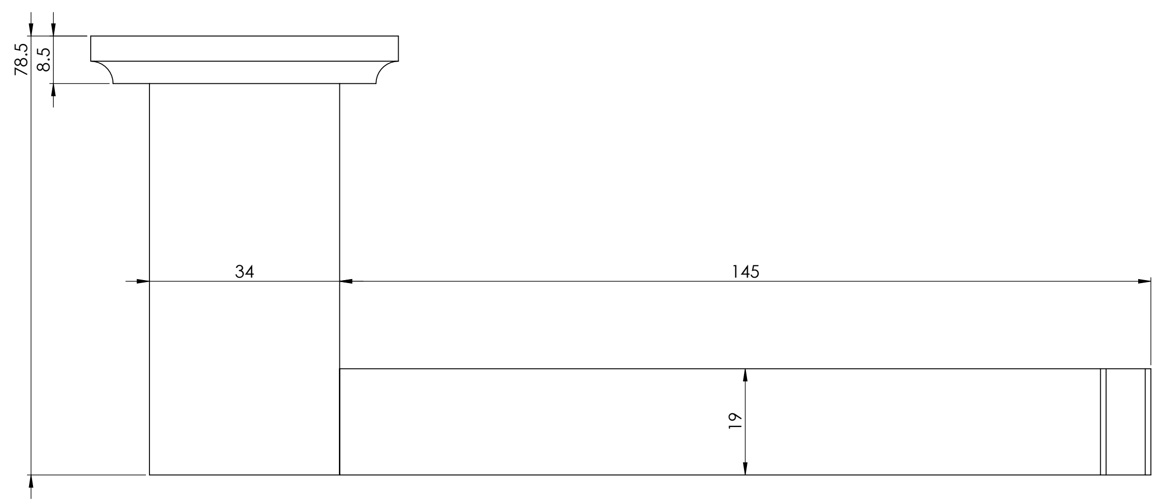
Top View
