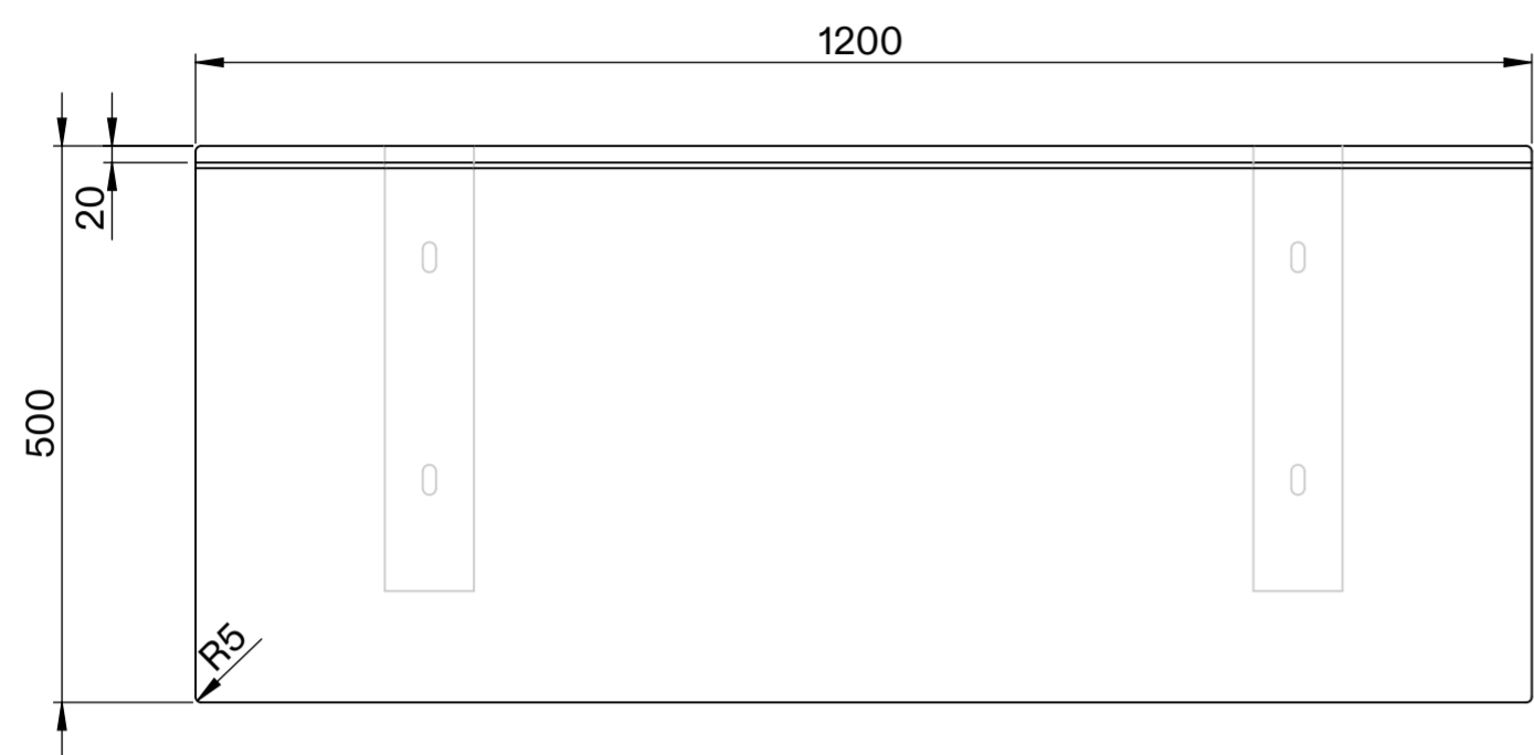
Top View
