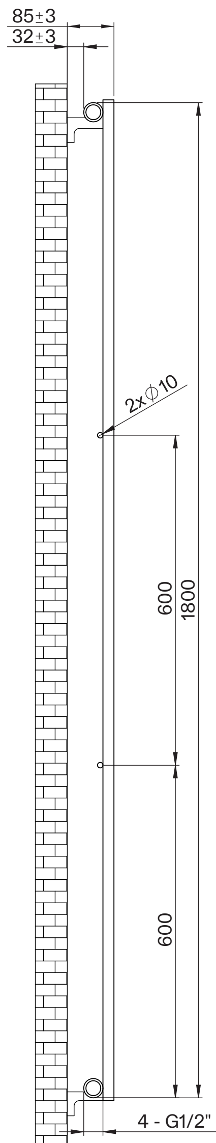
Side View
