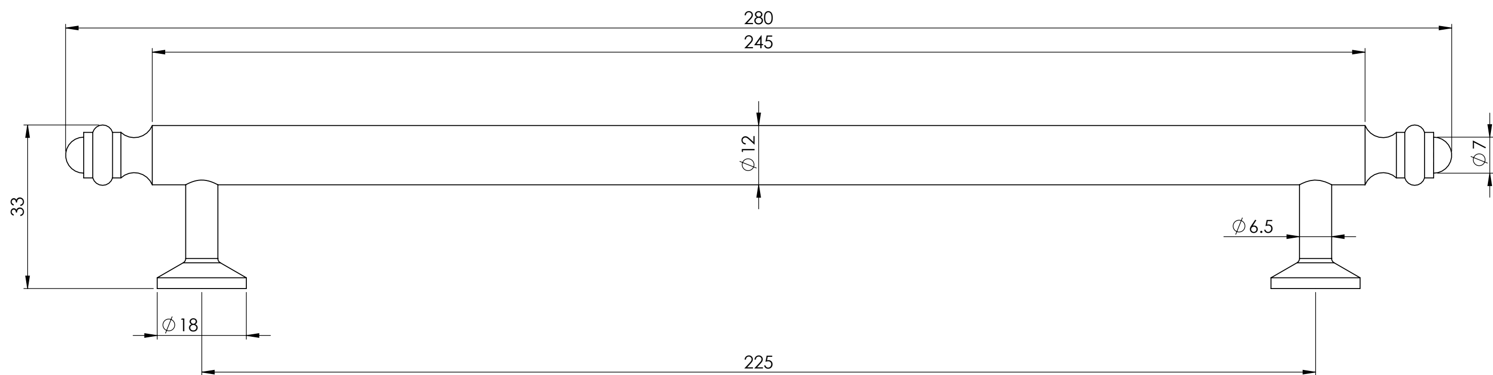
Top View
