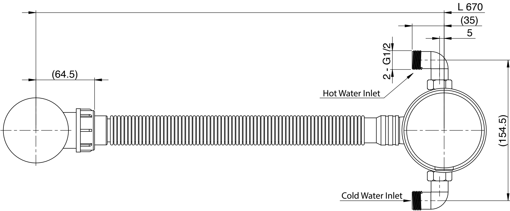
Top View
