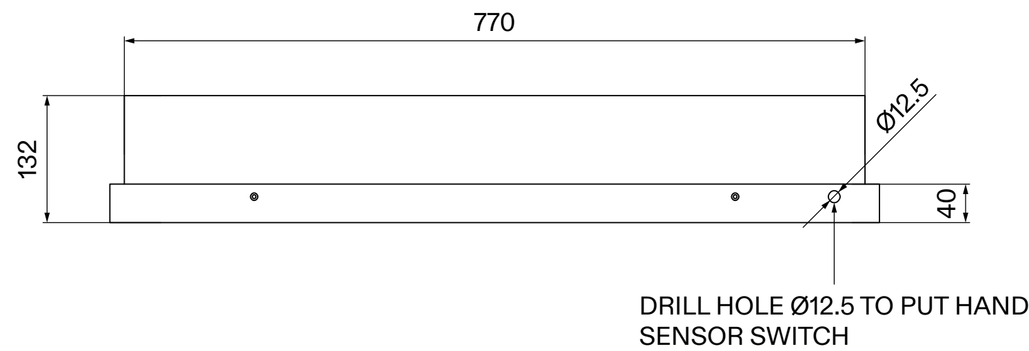
Bottom View
