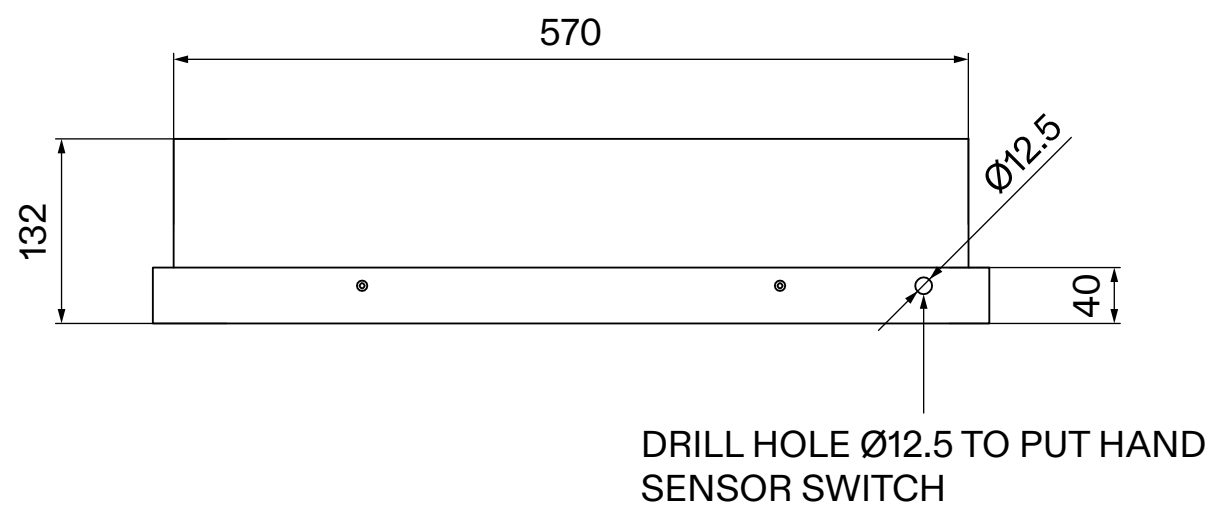
Bottom View
